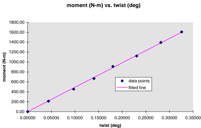
Figure 9. Load Test, Torsional Stiffness
