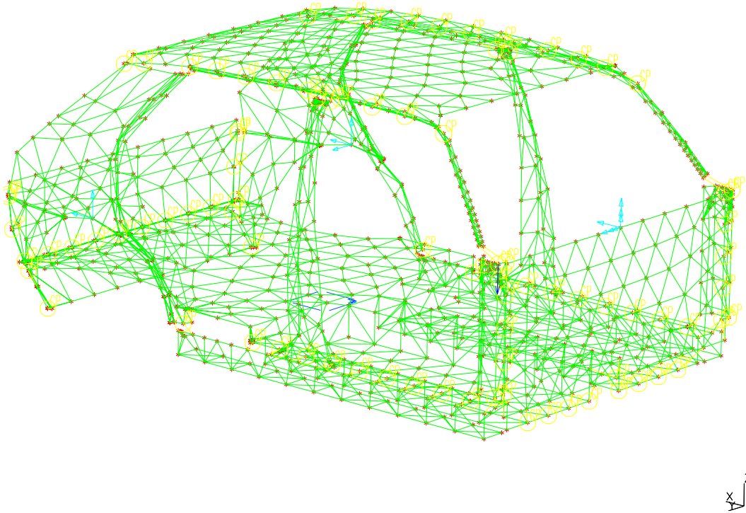
Figure 4. FINITE ELEMENT MODEL OF BODY-IN-WHITE
