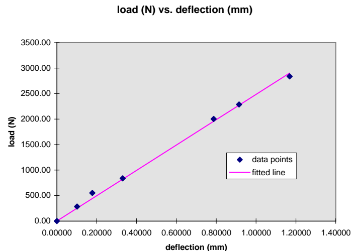
Figure 10. Load Test, Torsional Stiffness
