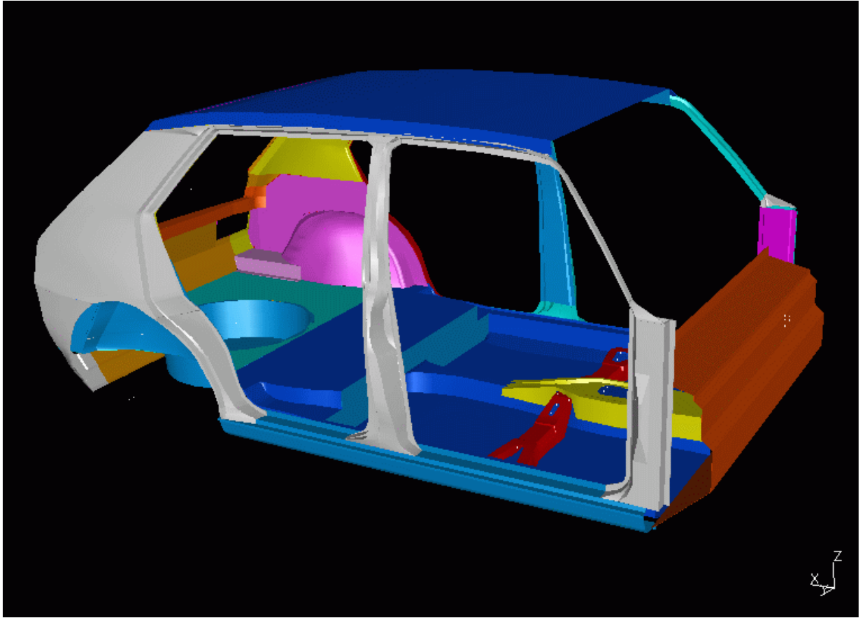
Figure 3. GEOMETRIC MODEL OF BODY-IN-WHITE IN SDRC I-DEAS
