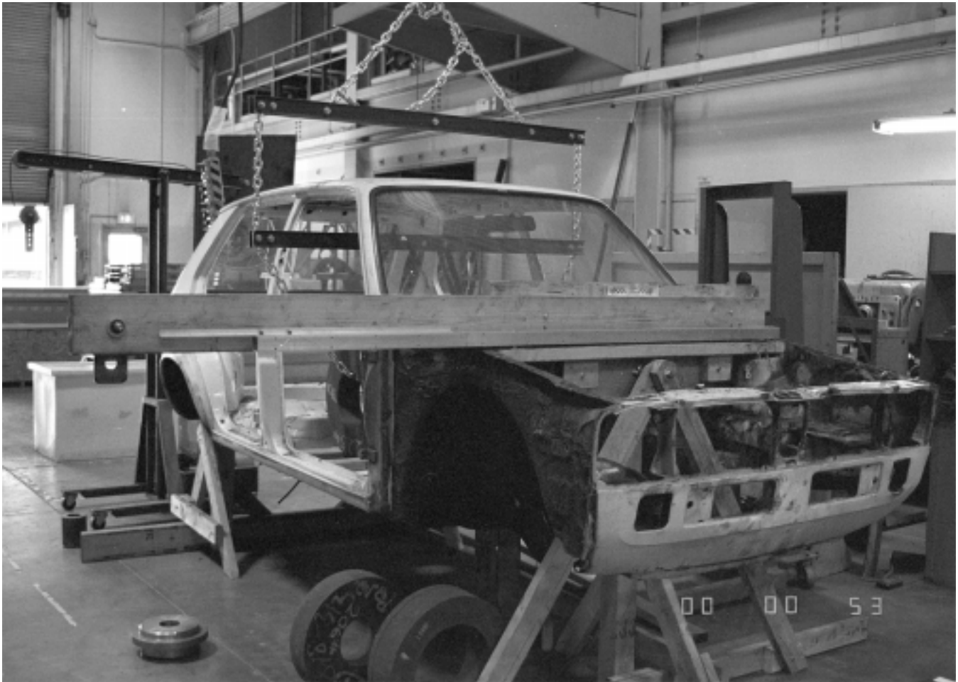
Figure 2. 1980 VW RABBIT IN STIFFNESS TESTING
